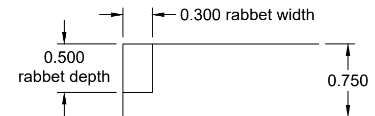
RABBET DETAIL
